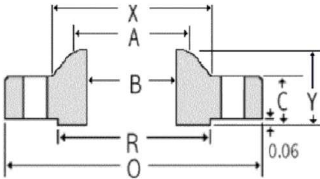
Weld Neck
