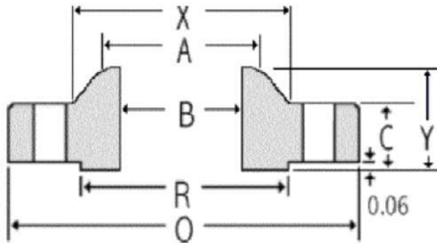
Weld Neck
